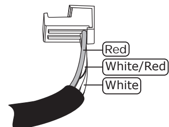
Temperature Cable Converter Assembly
