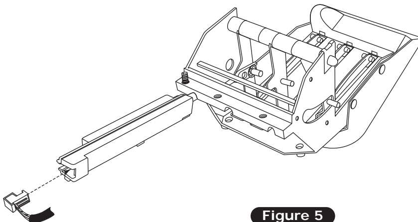
Temperature Cable Converter Assembly
