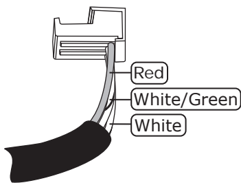
Blower Speed Cable Converter Assembly
