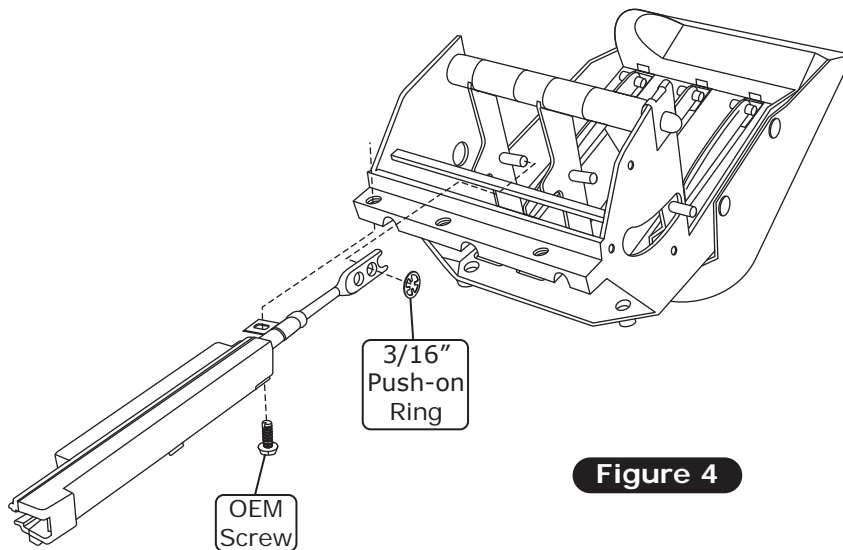
Rod Shown in Approximately Innermost Position
