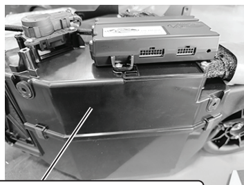
Route main wiring harness (white/yellow/purple) through wiring grommet on fresh air cap
