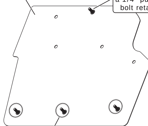
(3) 1/4-20 x 3/4" serrated flange black bolts and (3) 1/4" pushnut bolt retainer
